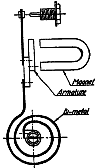
Thermostat Control
